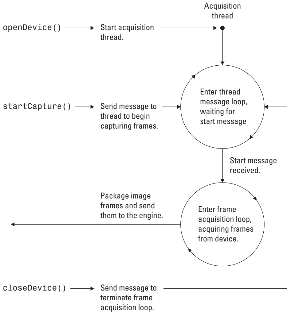
Interaction of Adaptor Functions and Acquisition Thread
